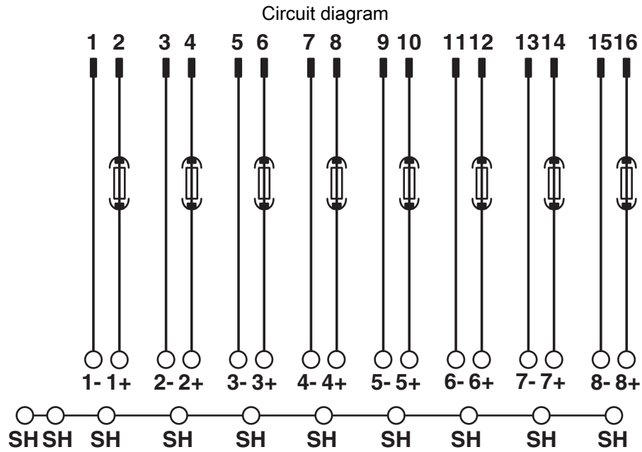
Connection scheme UM-DELTA/D/SI/BFI/TP
