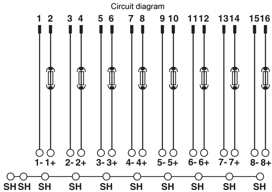
Connection scheme UM-DELTA V/D/SI/BFI/TP
