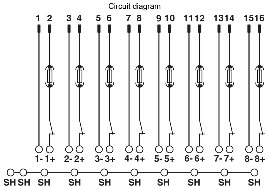
Connection scheme UM-DELTA/A/SI
