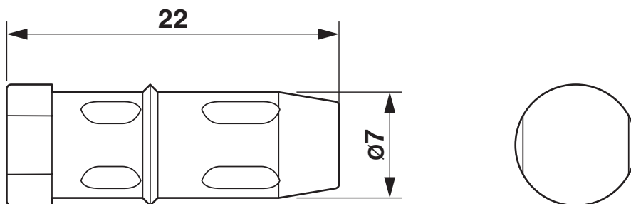
Dimensional drawing
