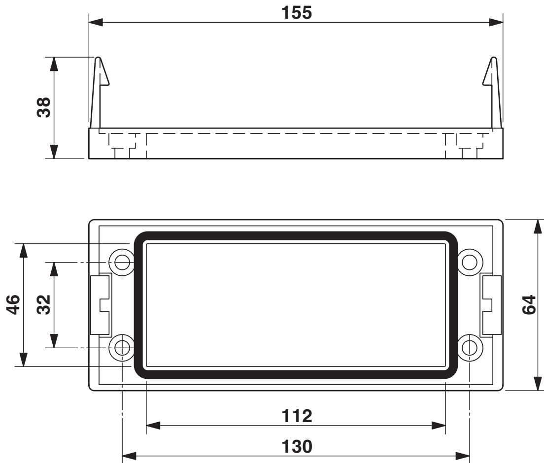
Dimensional drawing
