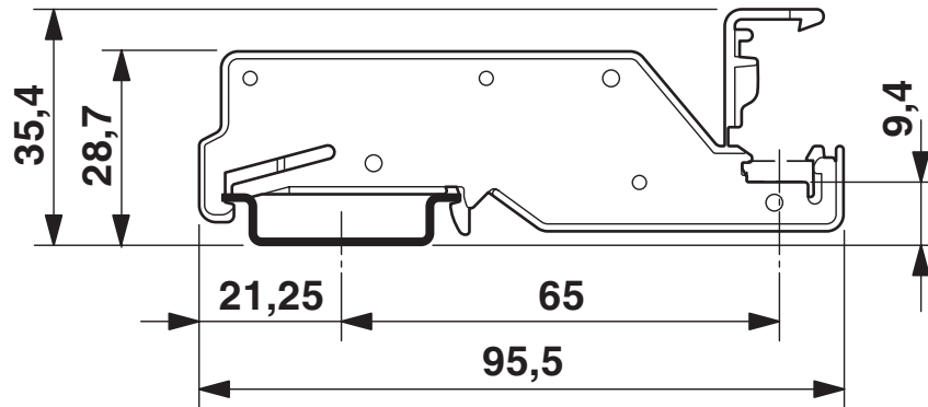
Dimensional drawing
