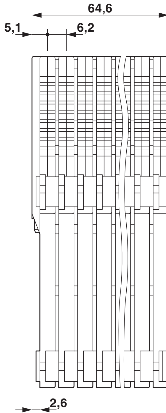
Dimensional drawing
