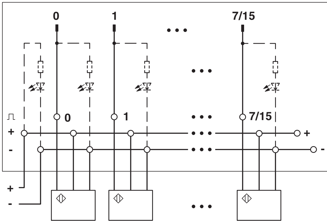
Circuit diagram
