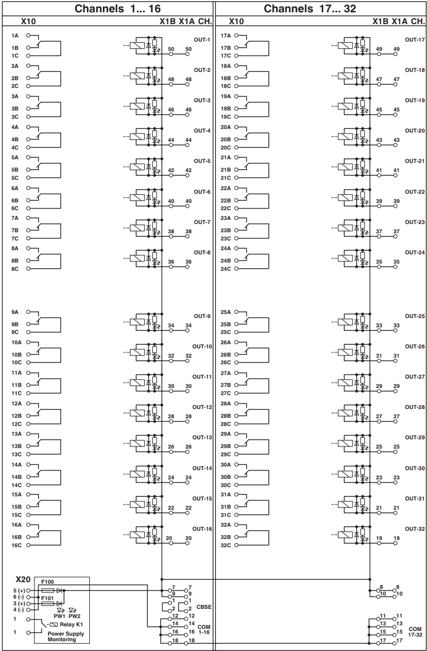
Circuit diagram
