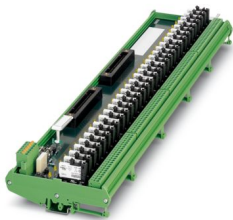
The figure shows a version UM-2KS50/32RM/MR/21/SPT/CS
