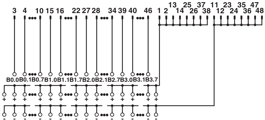
UM 45-FLK50/32IM/ZFKDS/PLC connection scheme
