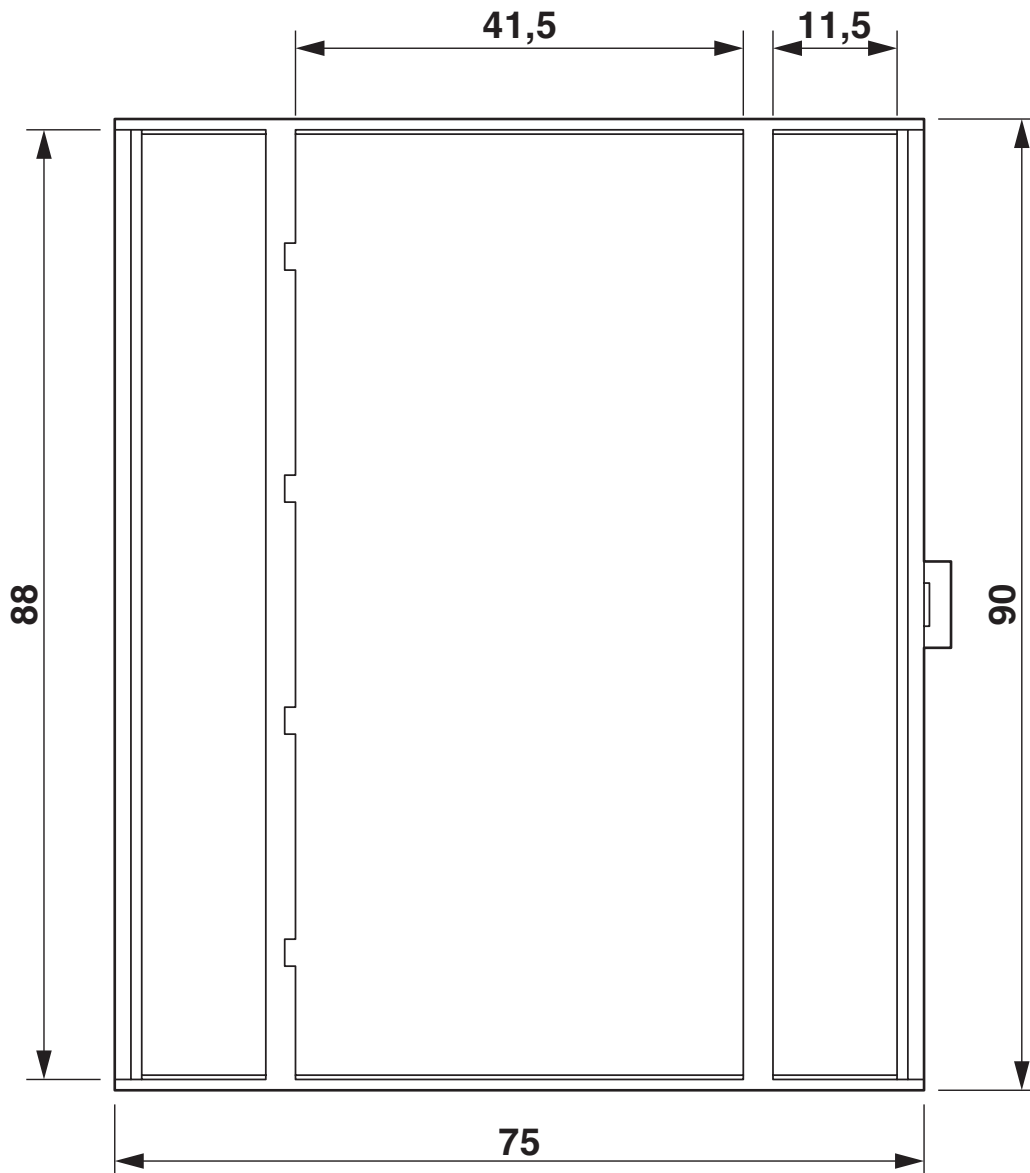
Dimensional drawing
