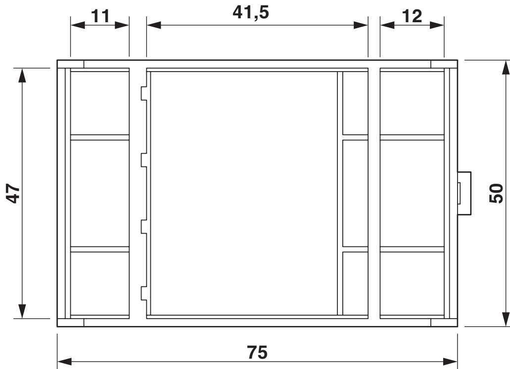
Dimensional drawing
