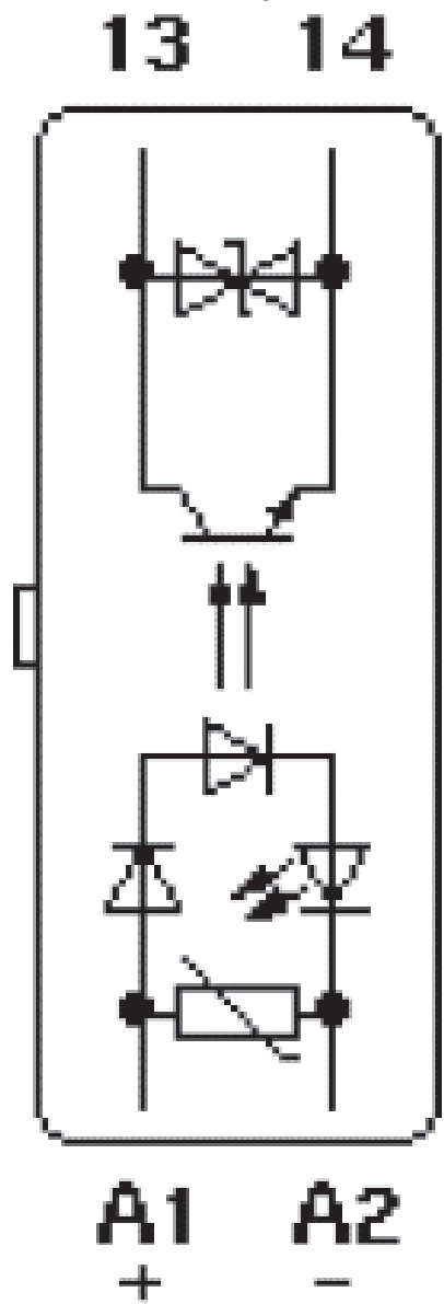
Circuit diagram
