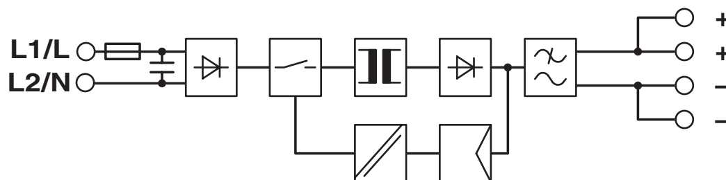
Block diagram
