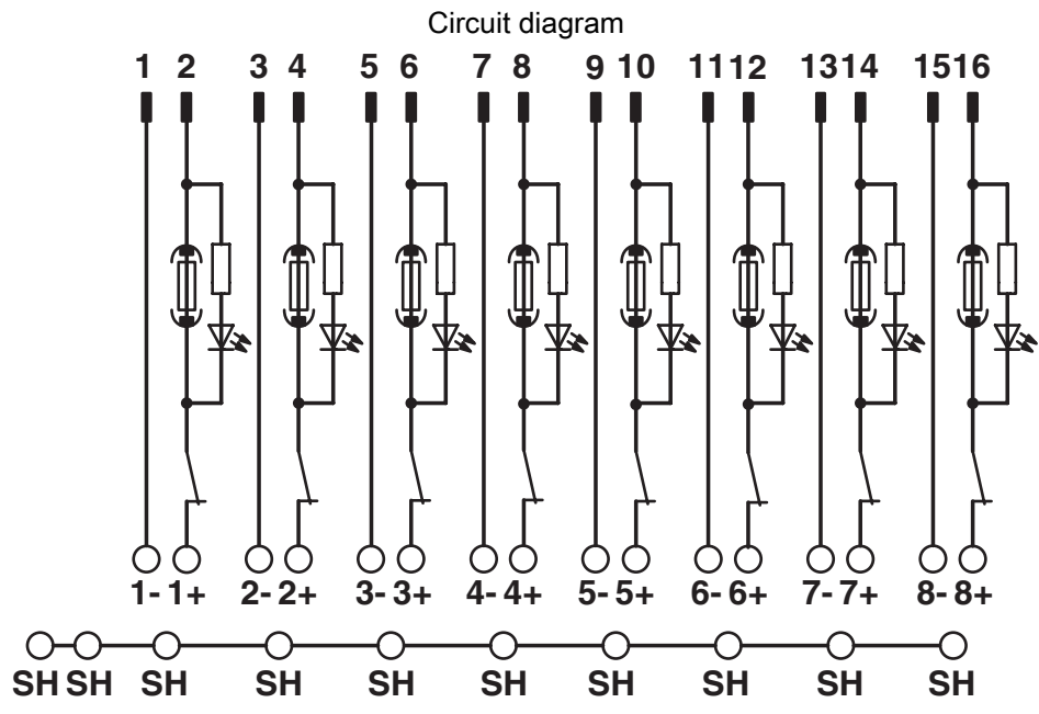
Connection scheme VIP-PT/FLK16/DS/FU/LED/AN/DV
