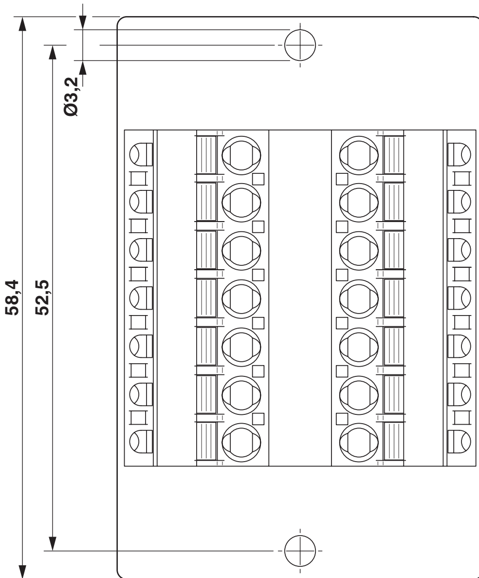
Dimensional drawing
