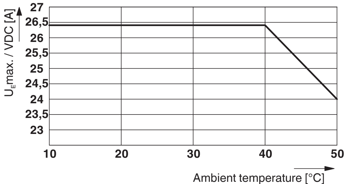
Derating curve for input voltage
