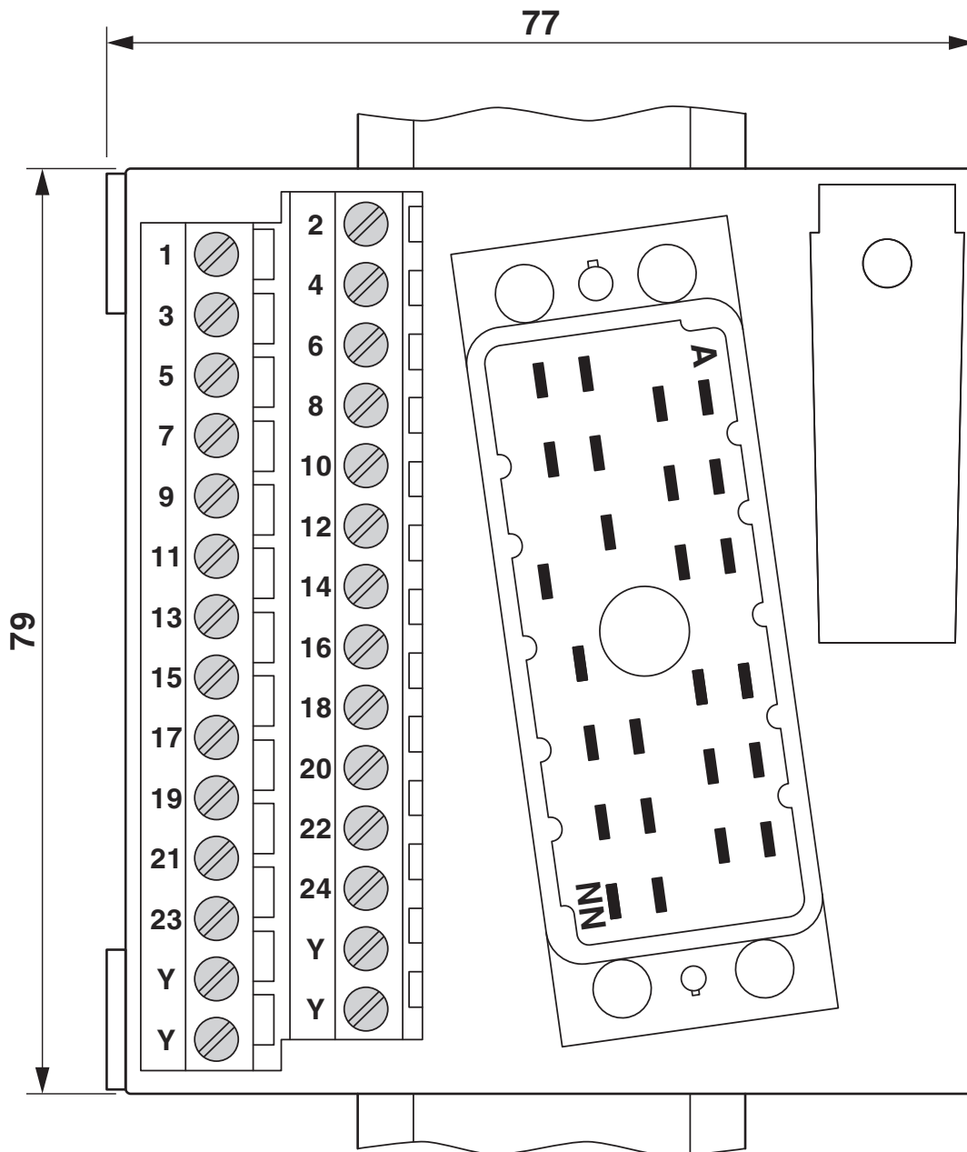
Dimensional drawing
