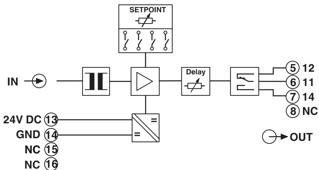
Circuit diagram
