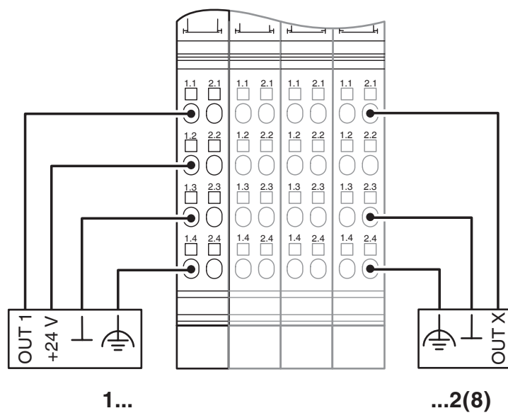
Connection diagram
