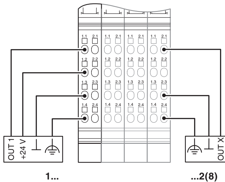
Connection diagram
