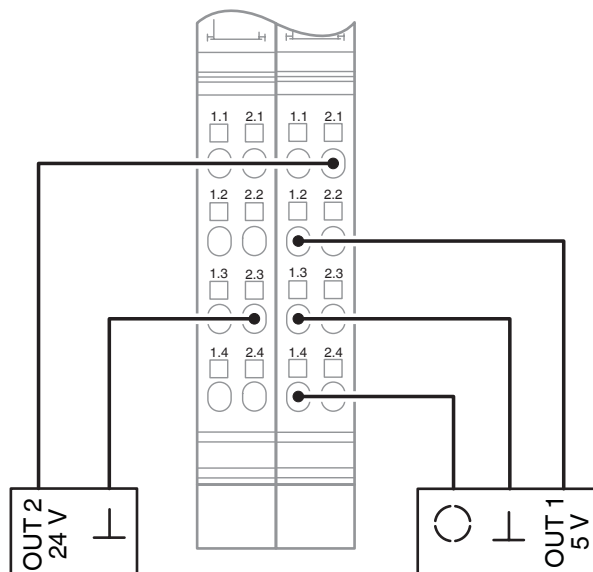
Connection diagram
