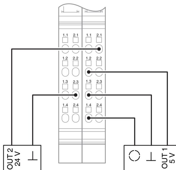
Connection diagram
