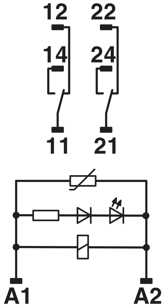
Circuit diagram
