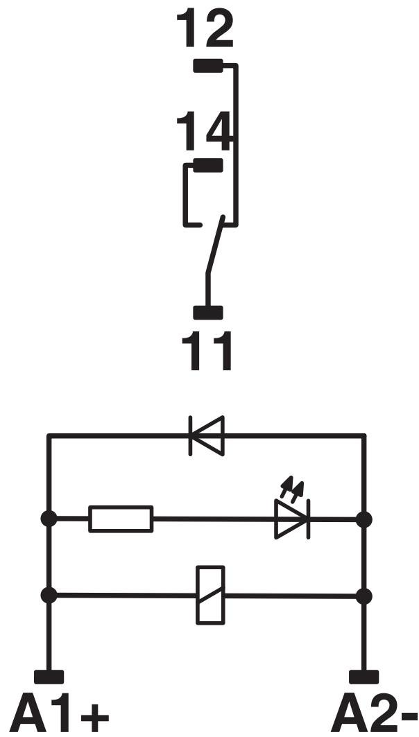
Circuit diagram
