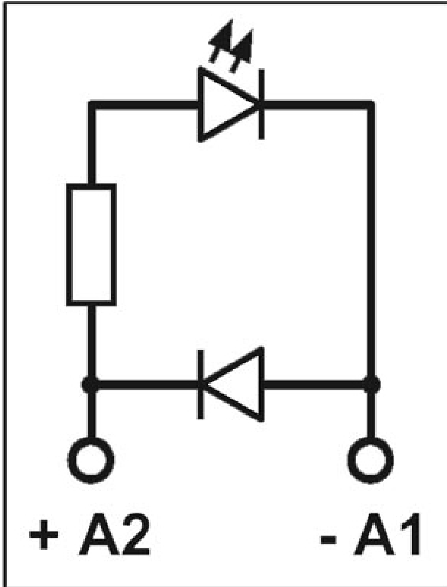
Circuit diagram
