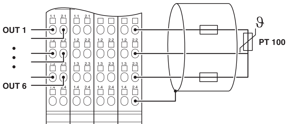
Connection diagram
