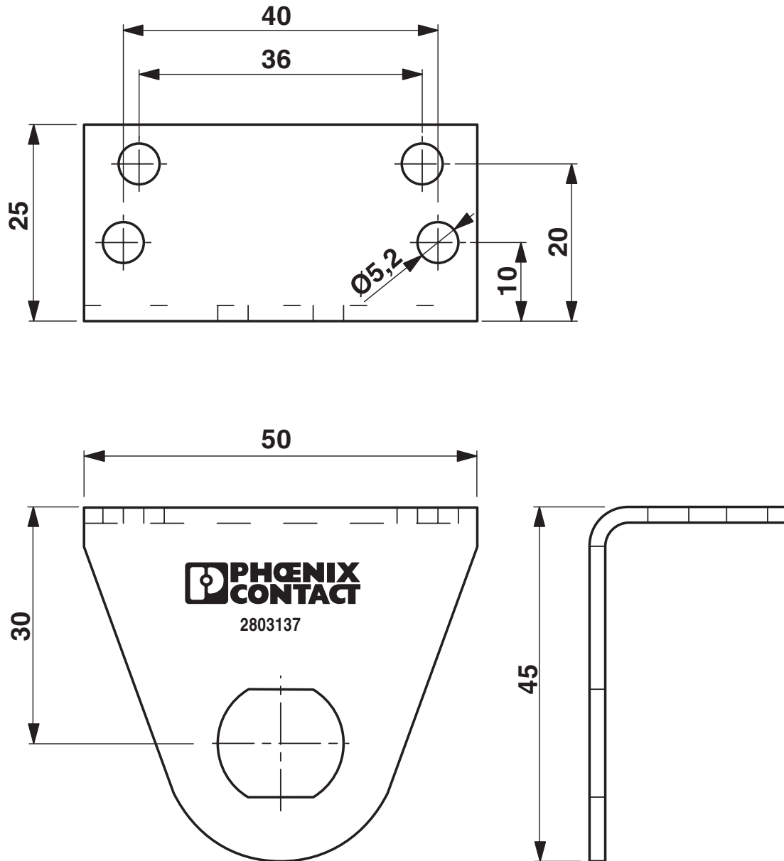
Dimensional drawing
