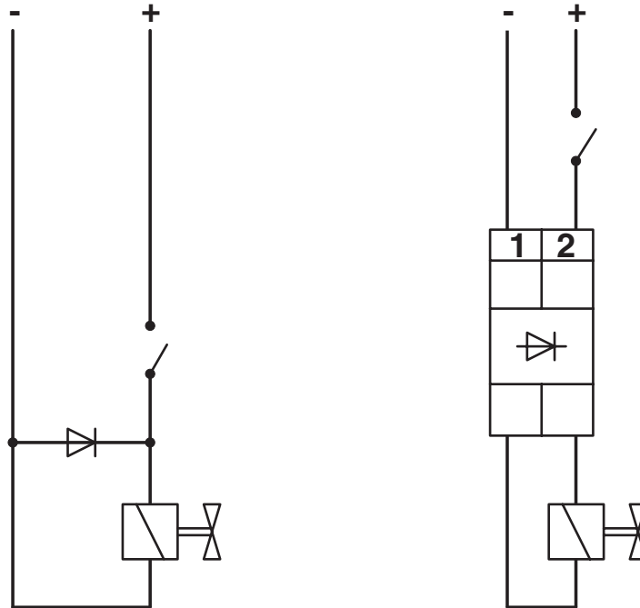
Circuit diagram
