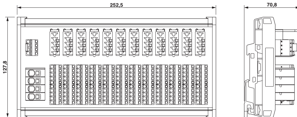
Dimensional drawing
