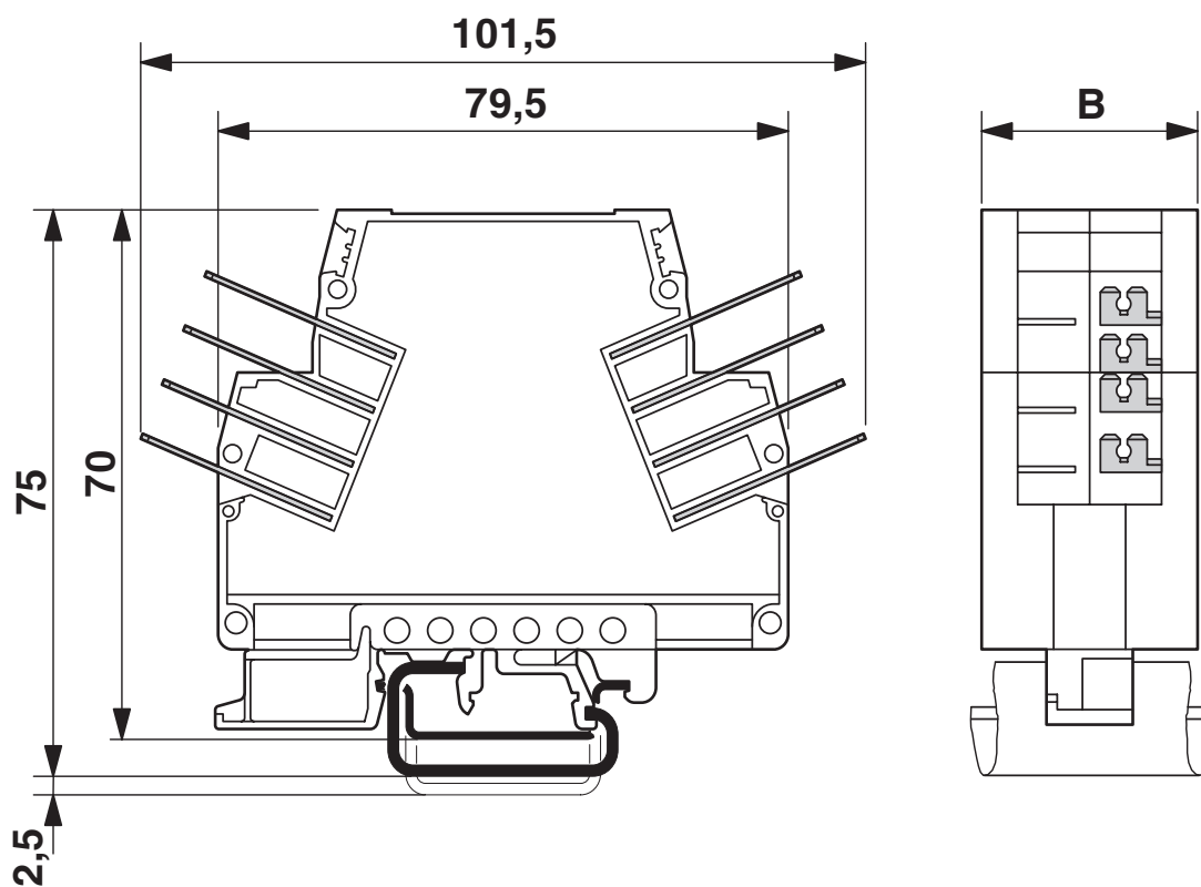
Dimensional drawing
