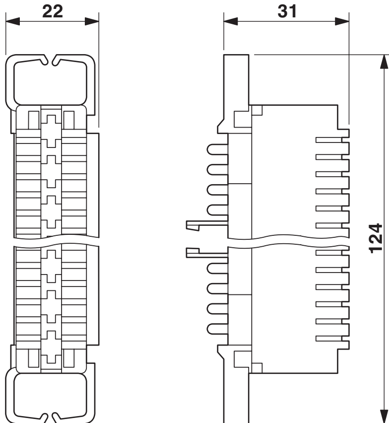
Dimensional drawing
