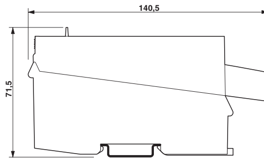
Dimensional drawing
