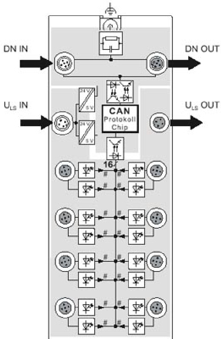
Block diagram
