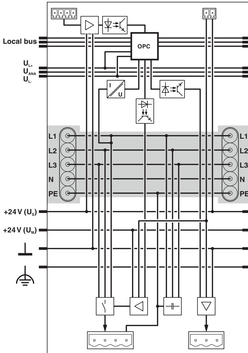
Block diagram
