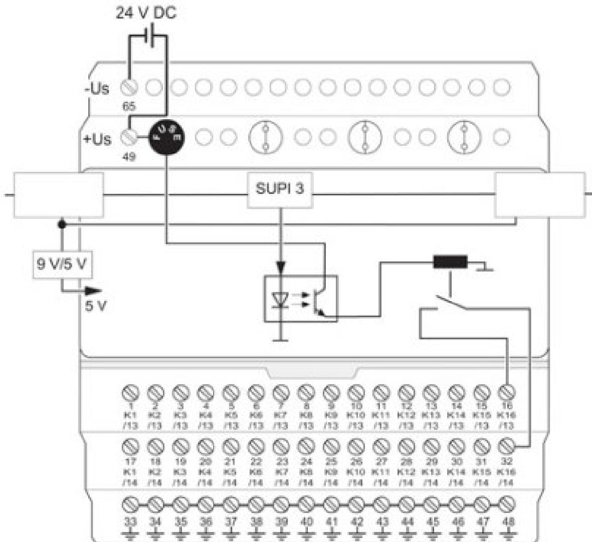
Block diagram
