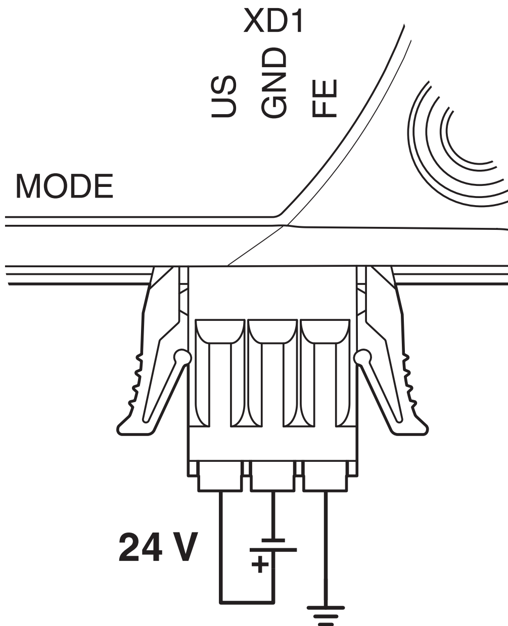
Connection diagram
