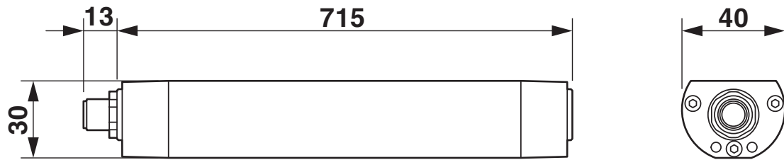
Dimensional drawing
