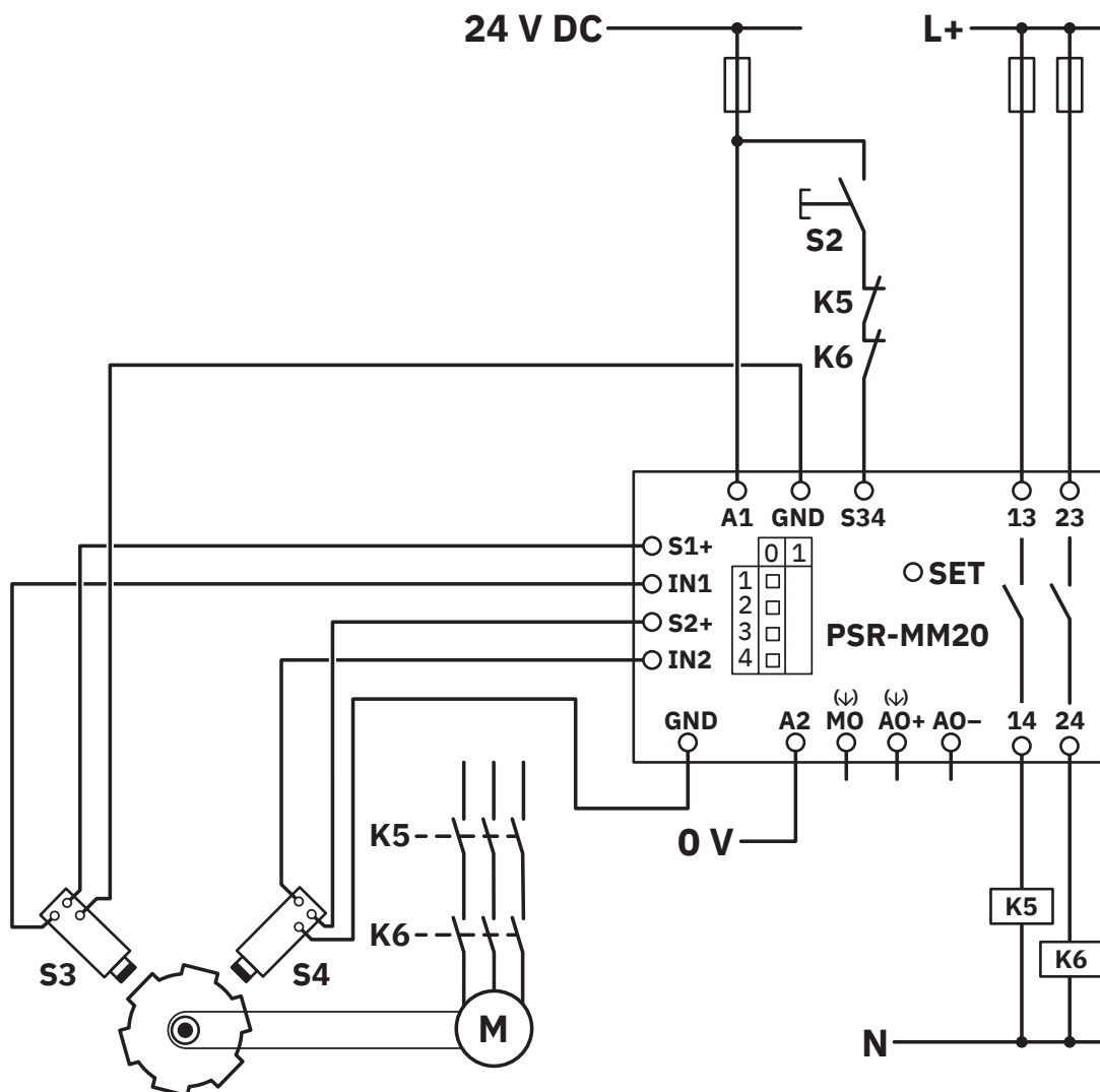
Circuit diagram
