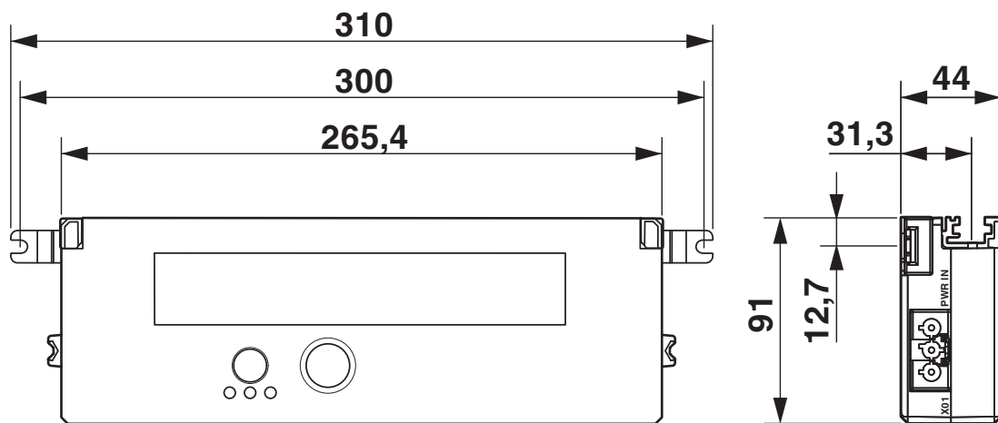
Dimensional drawing for screw mounting
