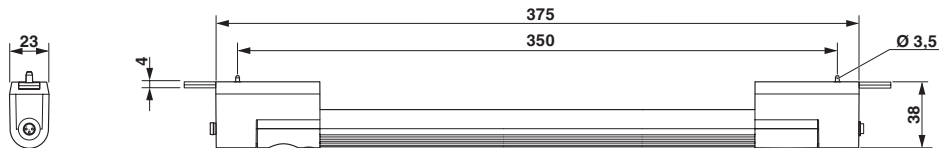
Dimensional drawing for screw mounting
