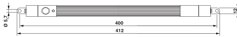
Dimensional drawing
