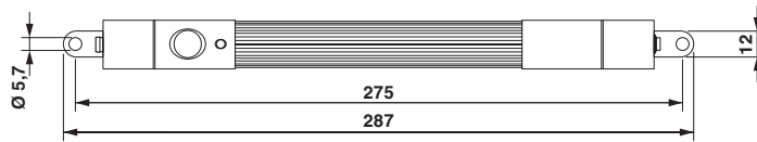
Dimensional drawing
