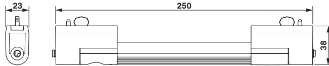
Dimensional drawing
