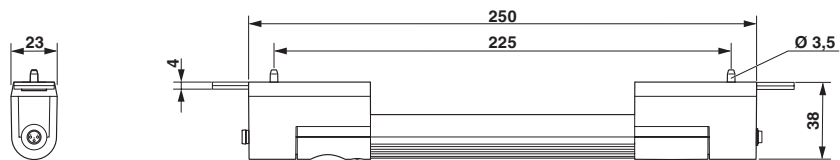
Dimensional drawing for screw mounting
