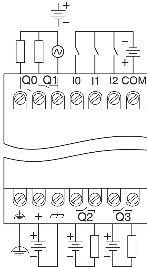
Connection diagram
