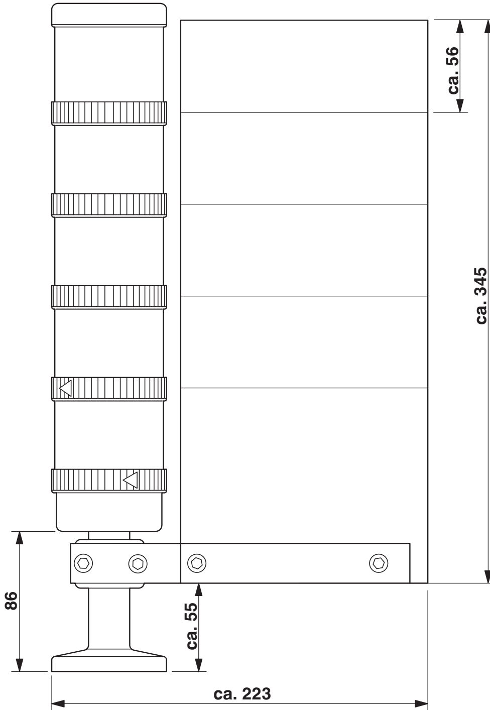
Dimensional drawing
