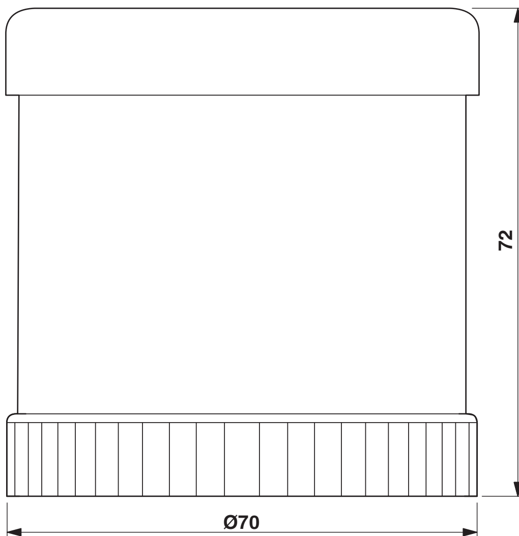
Dimensional drawing
