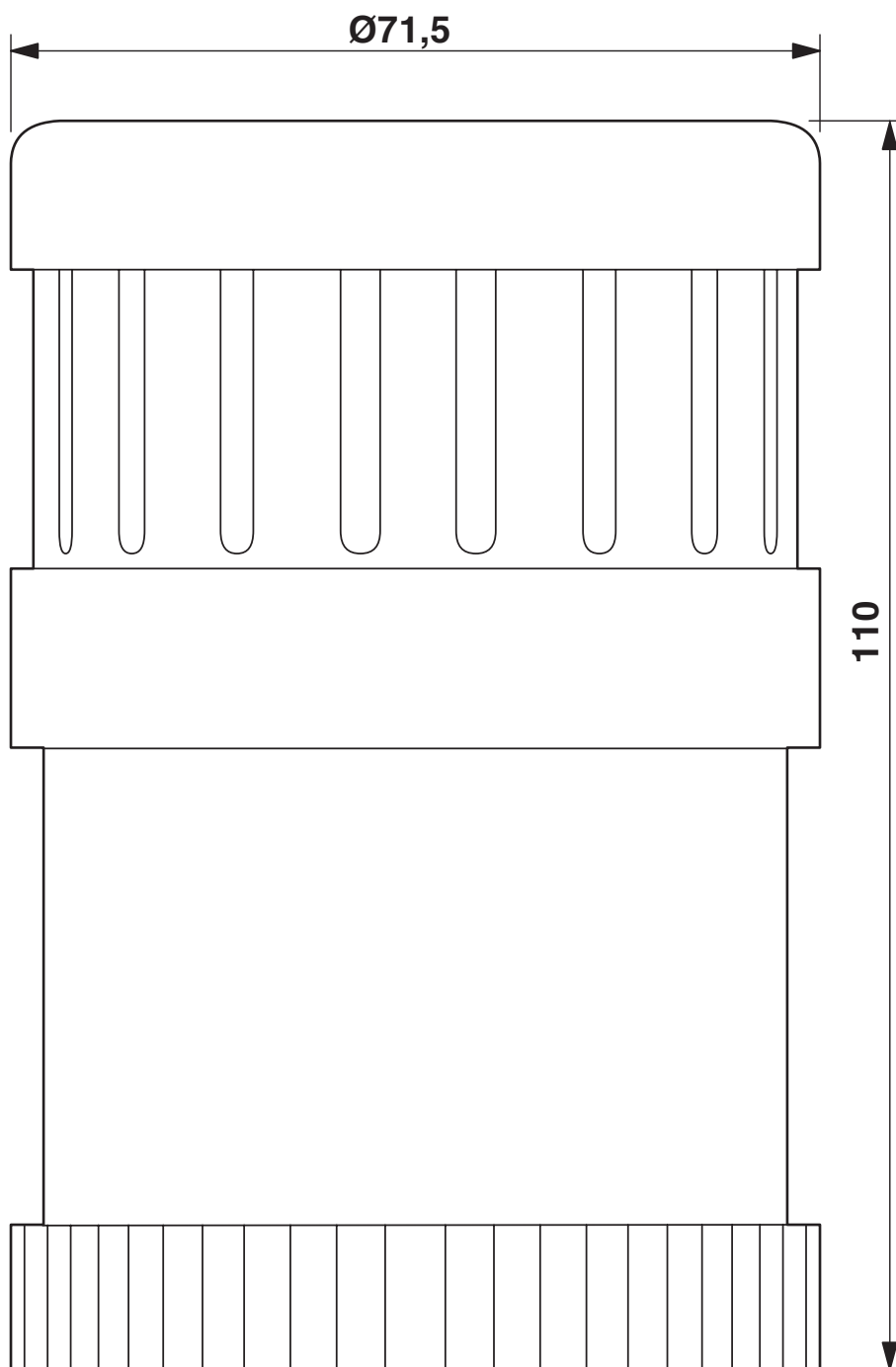
Dimensional drawing
