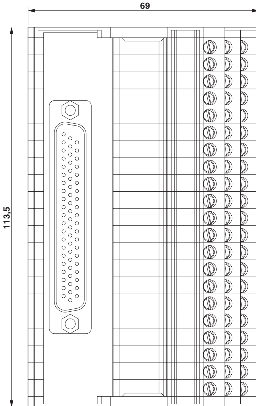
Dimensional drawing
