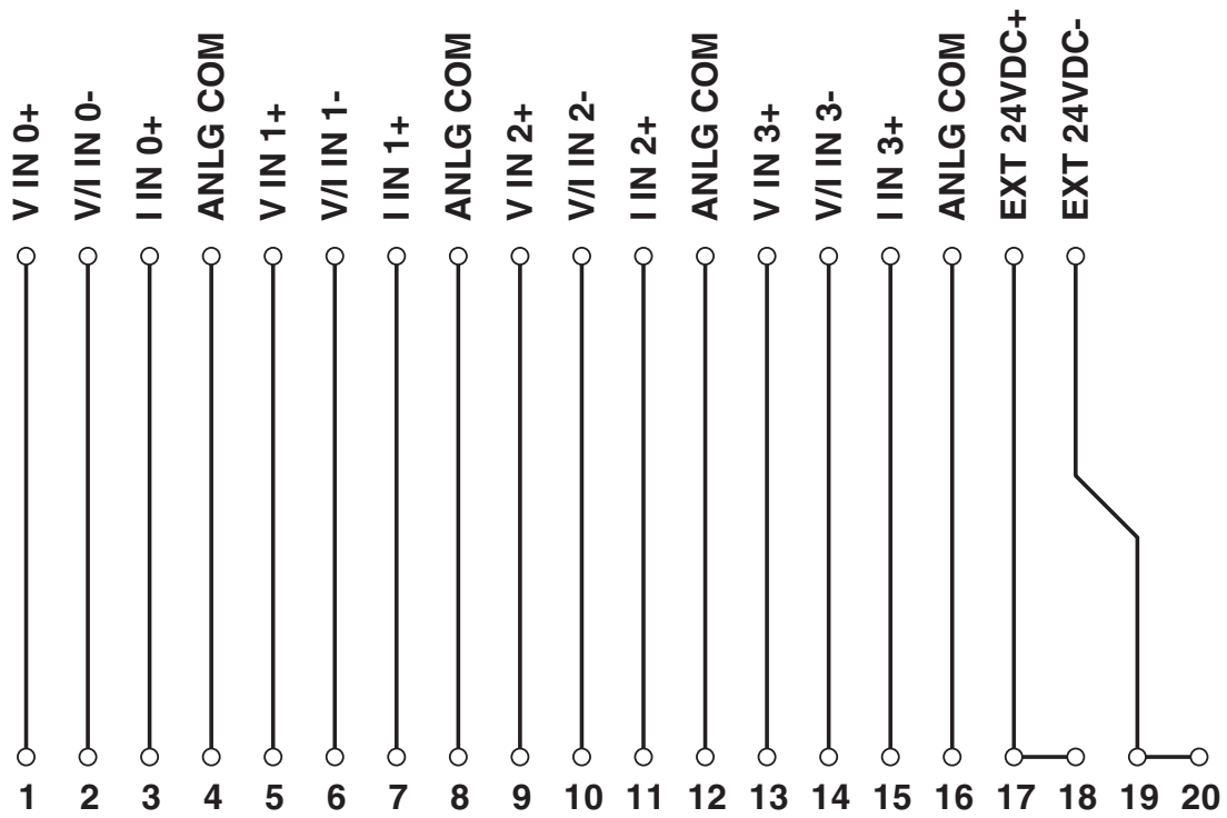
Circuit diagram
