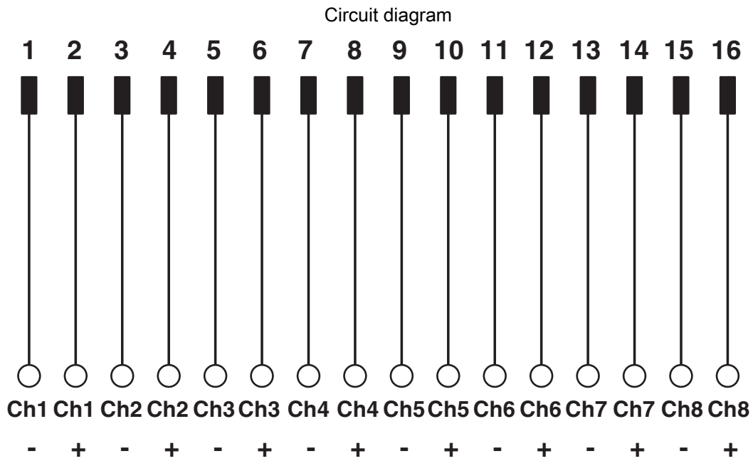
FLKM 16/DV connection scheme
