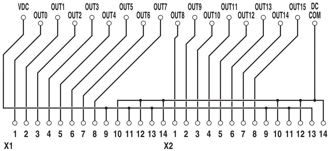
Circuit diagram
