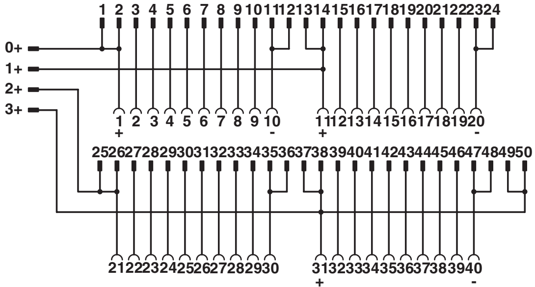
Connection scheme FLKM 50-PA-AB/OBN
