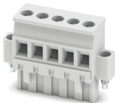
The figure shows version MVSTBR 2,5/ 5-STF-5,08 AU
