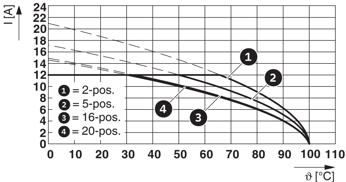
Type: FKCT 2,5/...-ST with MSTBV 2,5/...-G
